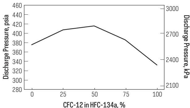
Figure 2. Effect of Increasing Concentrations of CFC-12 in Freon™ 134a on Compressor Discharge Pressure (Condenser at 79 °C [175 °F]; Evaporator at 4.5 °C [40 °F])
